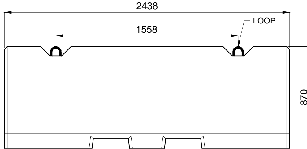
ELEVATION VIEW
