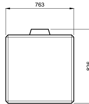
SIDE ELEVATION
